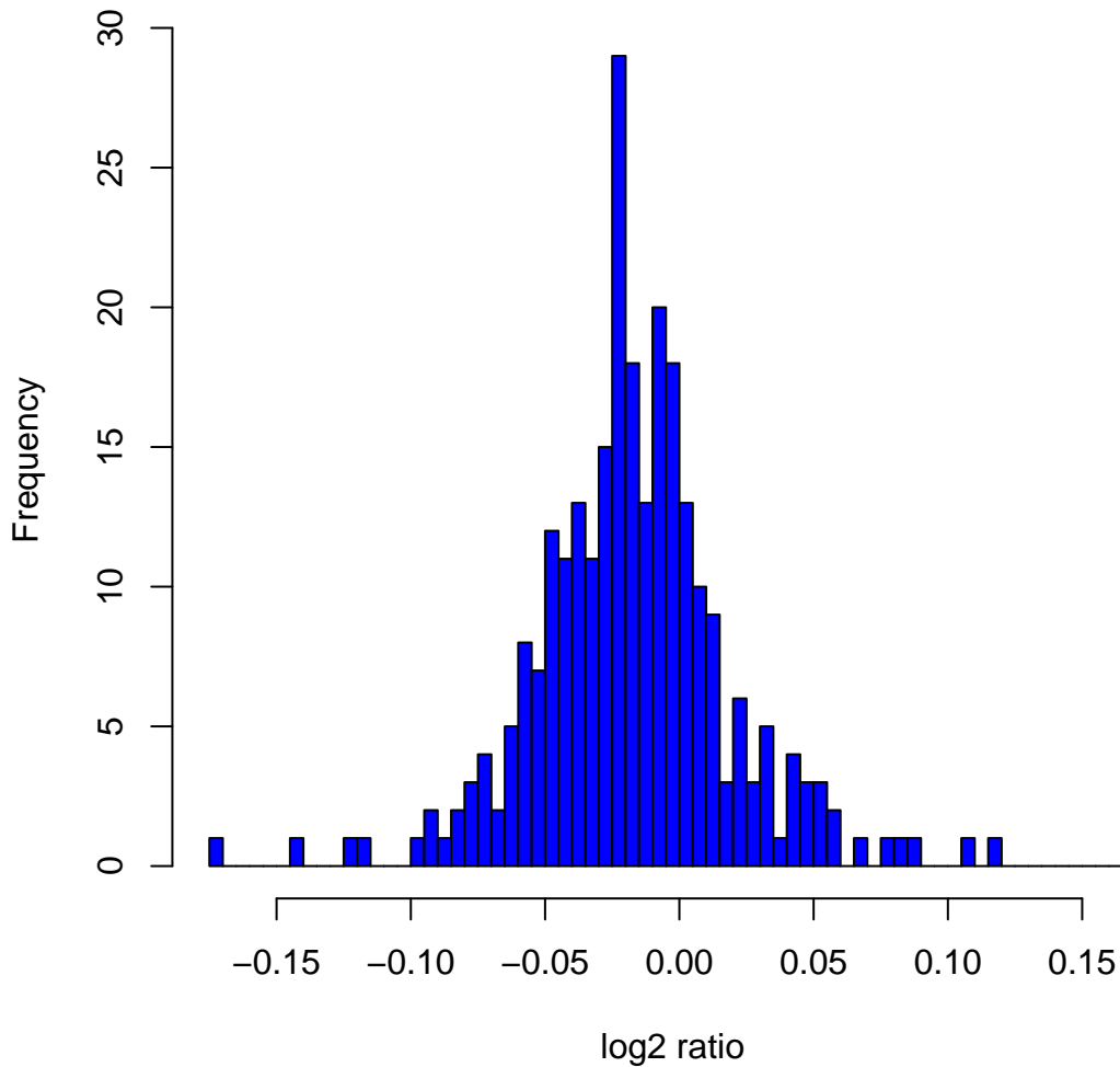
Histogram of \log_2 ratios in 270 HapMap samples at clone Chr20tp-3A9
