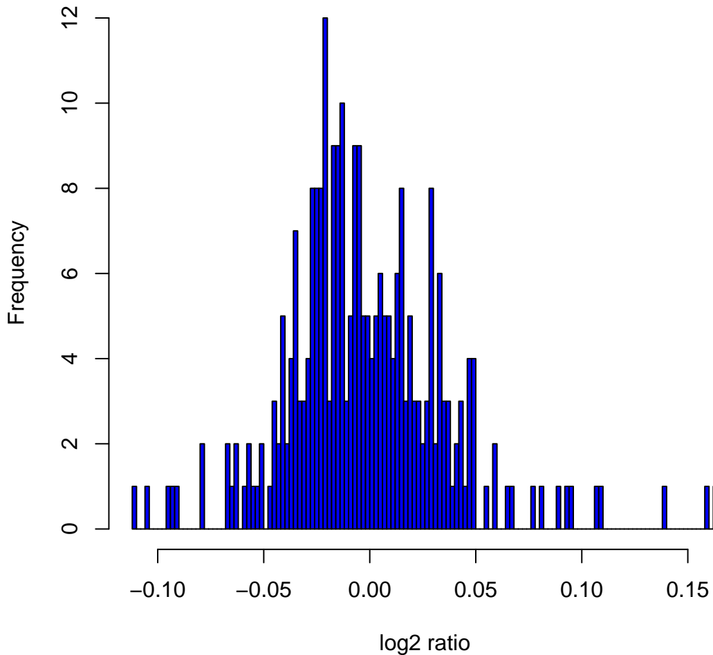
Histogram of log 2 ratios in 270 HapMap samples at clone Chr20tp-3C8
