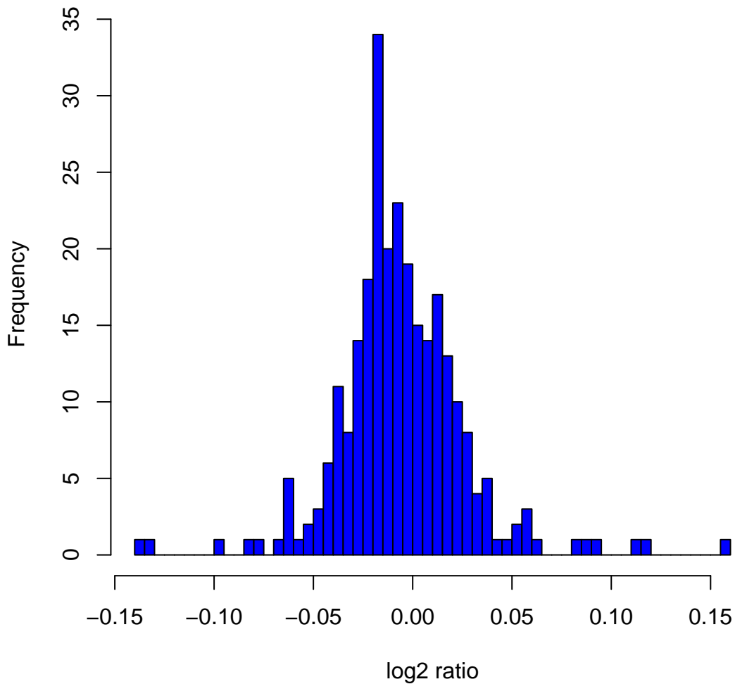
Histogram of log 2 ratios in 270 HapMap samples at clone Chr20tp-3E1
