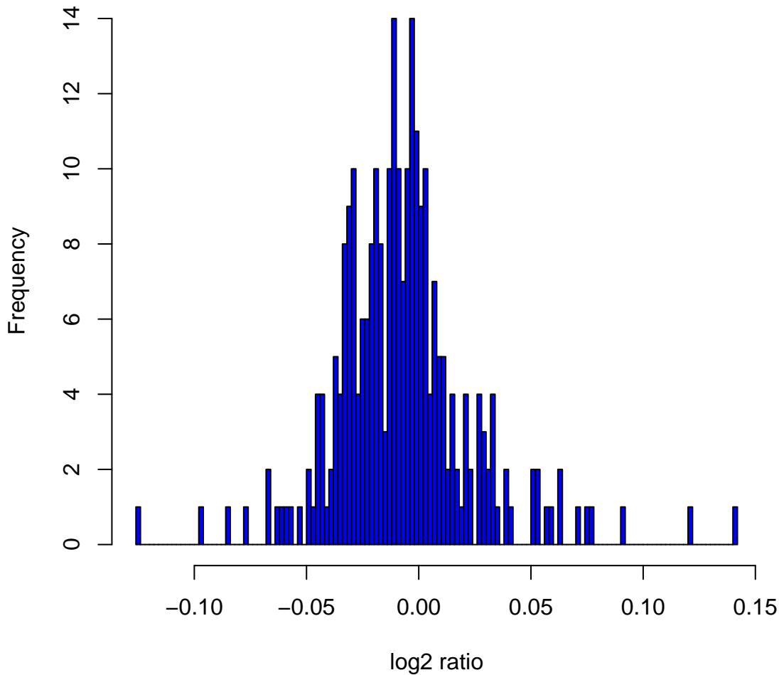
Histogram of log2ratios in 270 HapMap samples at clone Chr20tp-3G12
