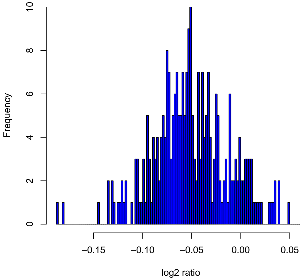
Histogram of log 2 ratios in 270 HapMap samples at clone Chr20tp-3G8
