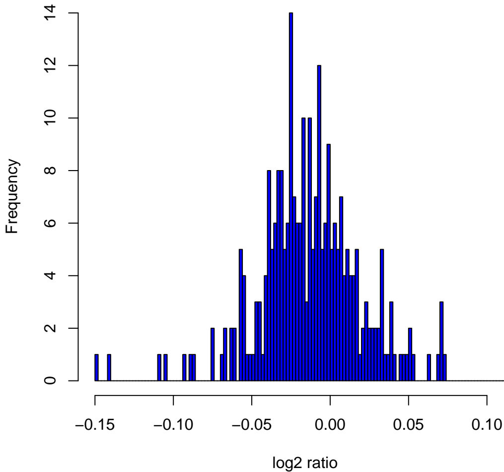
Histogram of log 2 ratios in 270 HapMap samples at clone Chr20tp-5A6
