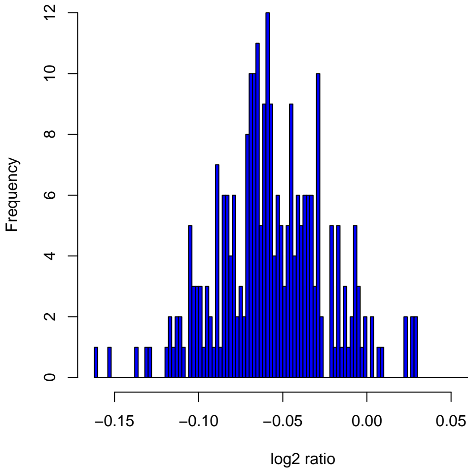
Histogram of log2ratios in 270 HapMap samples at clone Chr20tp-5C10
