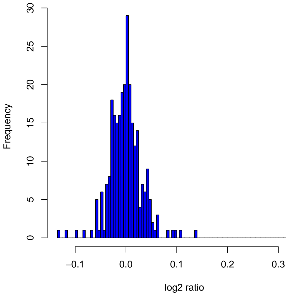
Histogram of log 2 ratios in 270 HapMap samples at clone Chr20tp-5C4
