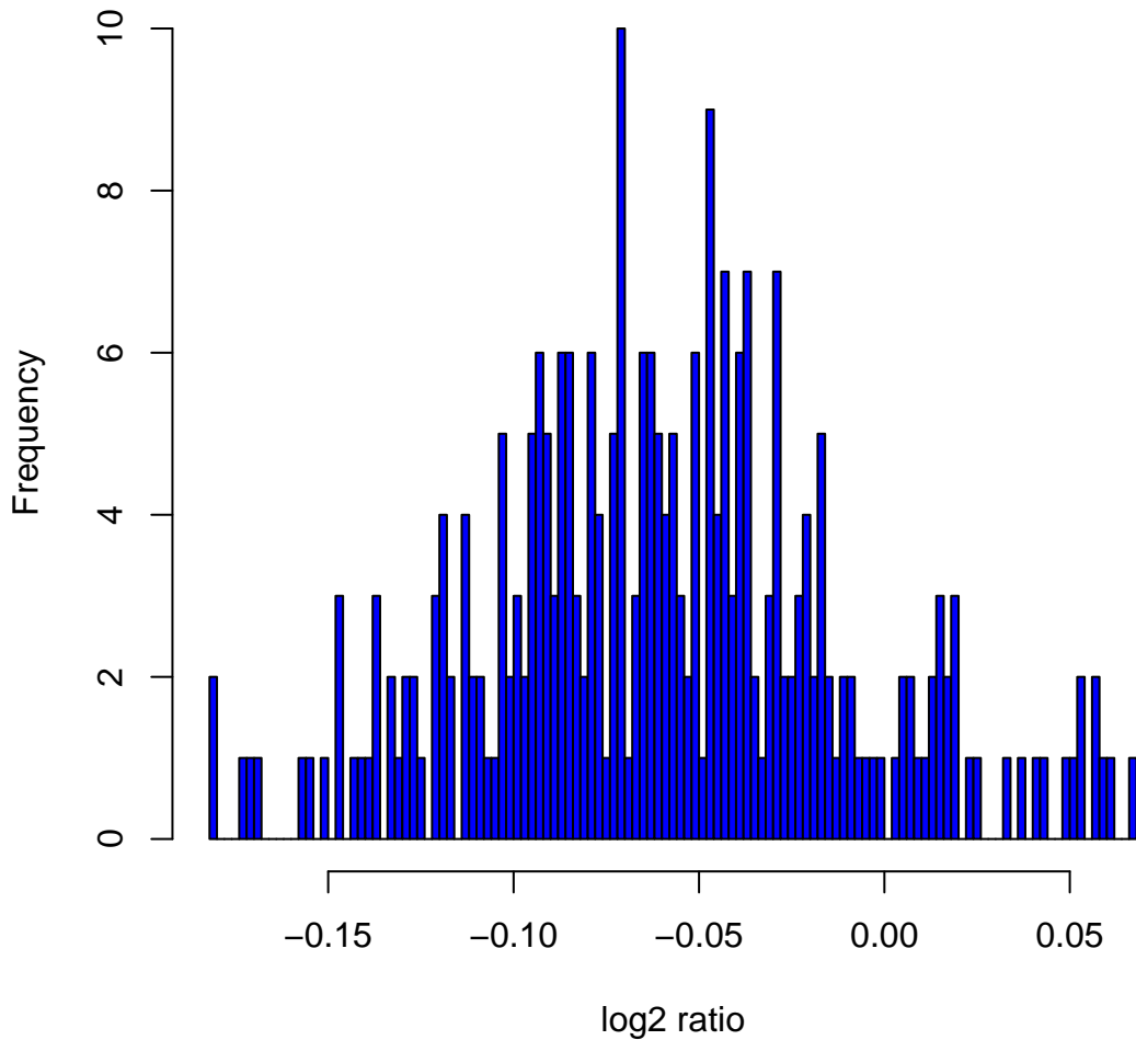
Histogram of log 2 ratios in 270 HapMap samples at clone Chr20tp-5D3
