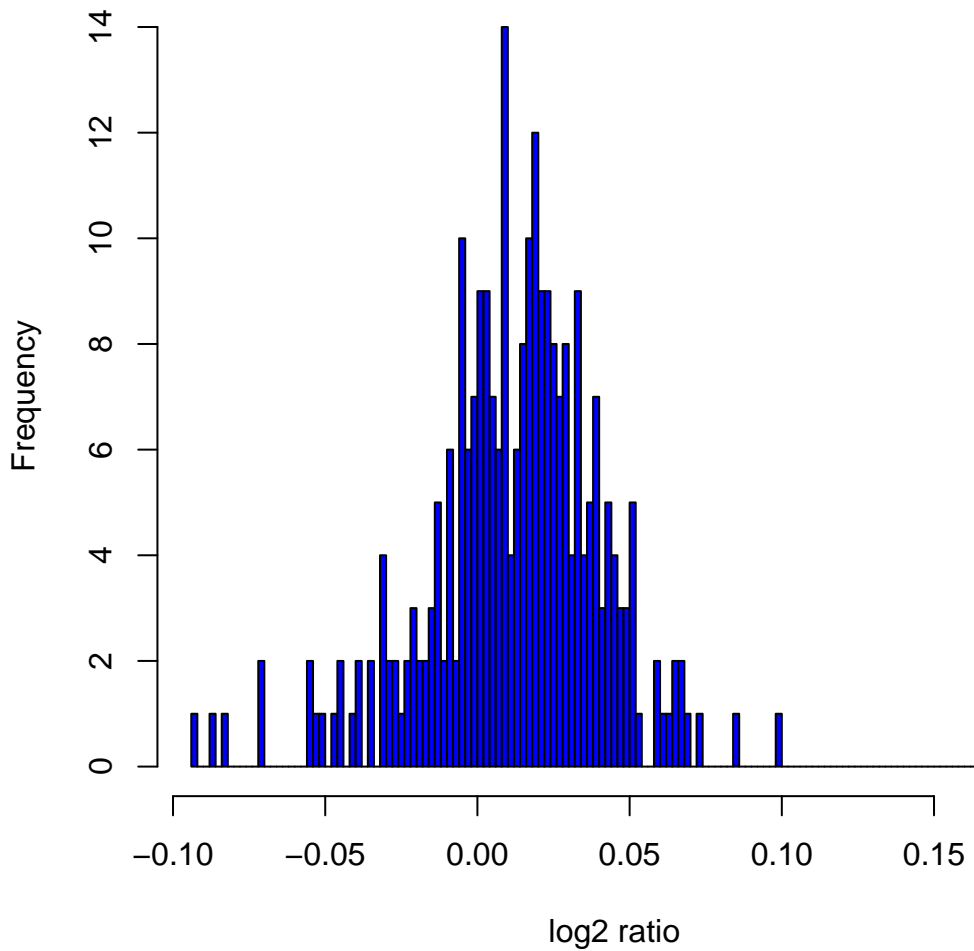
Histogram of log 2 ratios in 270 HapMap samples at clone Chr20tp-5E3
