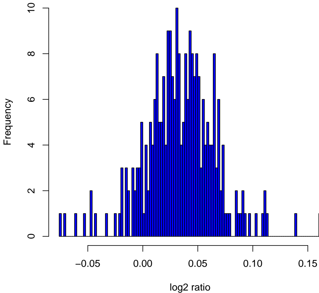
Histogram of log2ratios in 270 HapMap samples at clone Chr20tp-5F12
