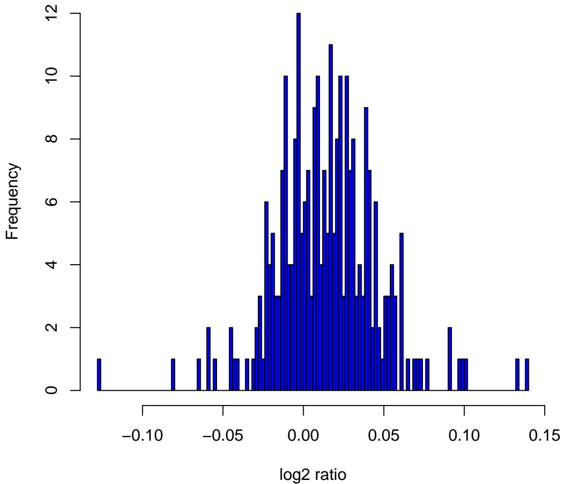
Histogram of log2ratios in 270 HapMap samples at clone Chr20tp-5G11
