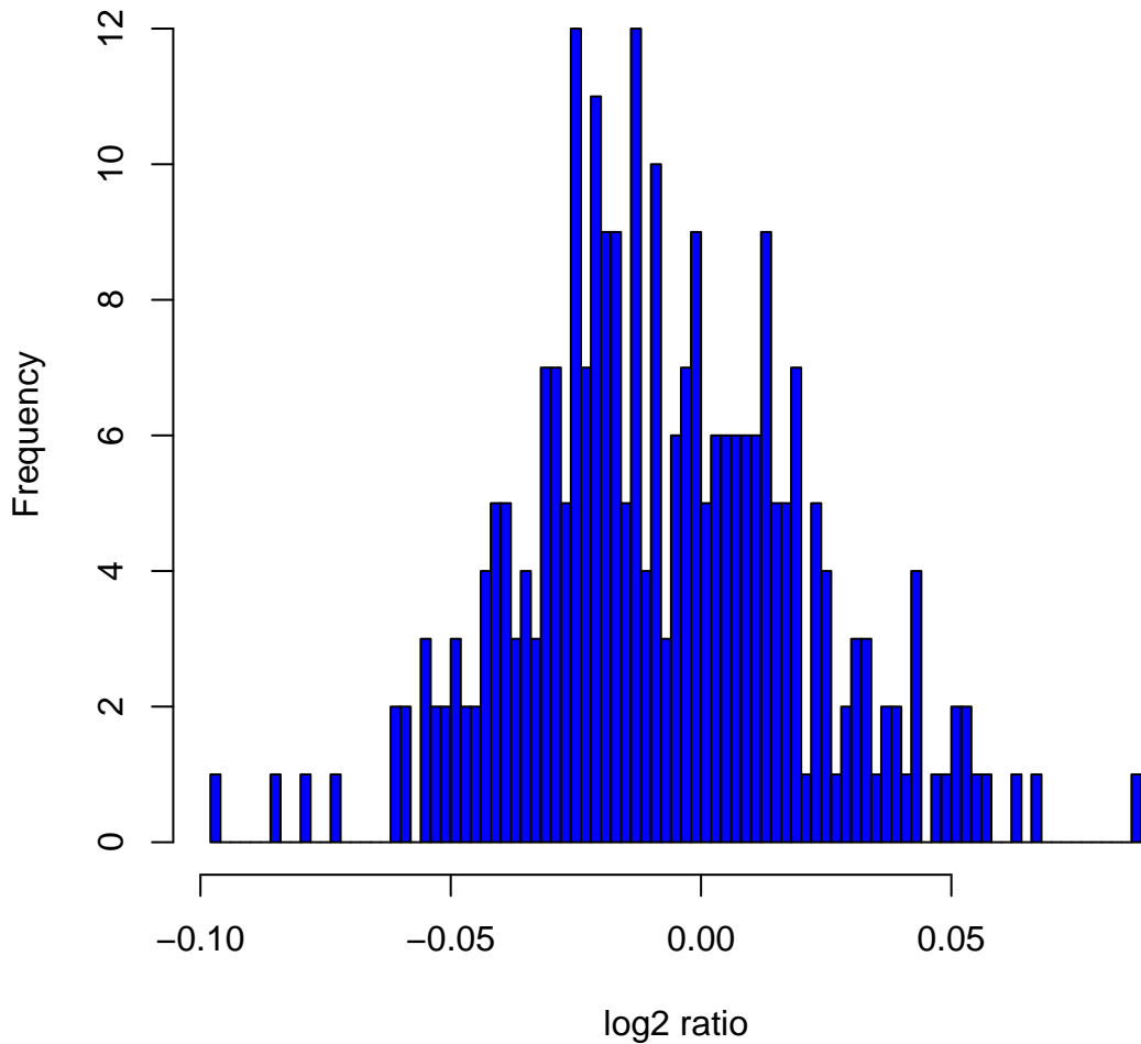
Histogram of log2ratios in 270 HapMap samples at clone Chr20tp-5G12
