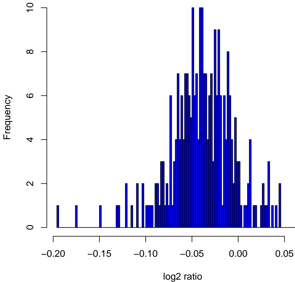
Histogram of log2ratios in 270 HapMap samples at clone Chr20tp-5G5
