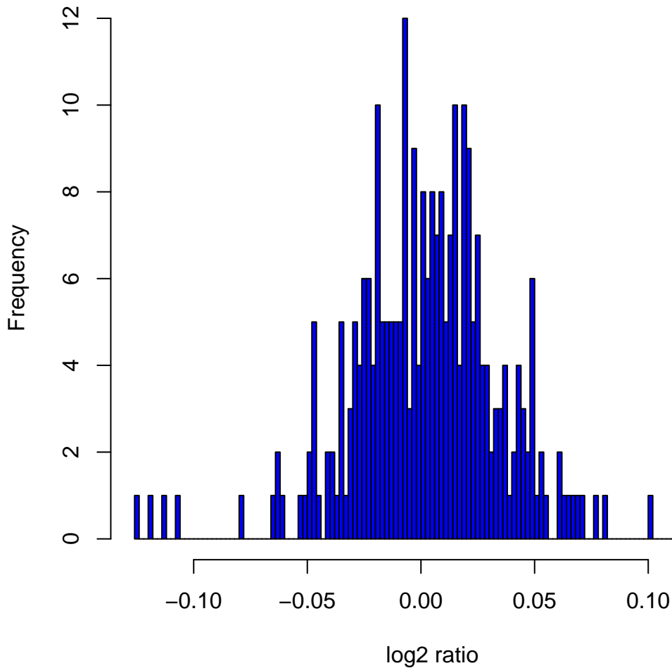
Histogram of log2ratios in 270 HapMap samples at clone Chr20tp-6A12
