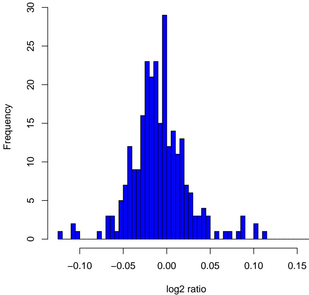
Histogram of log2ratios in 270 HapMap samples at clone Chr20tp-6C9
