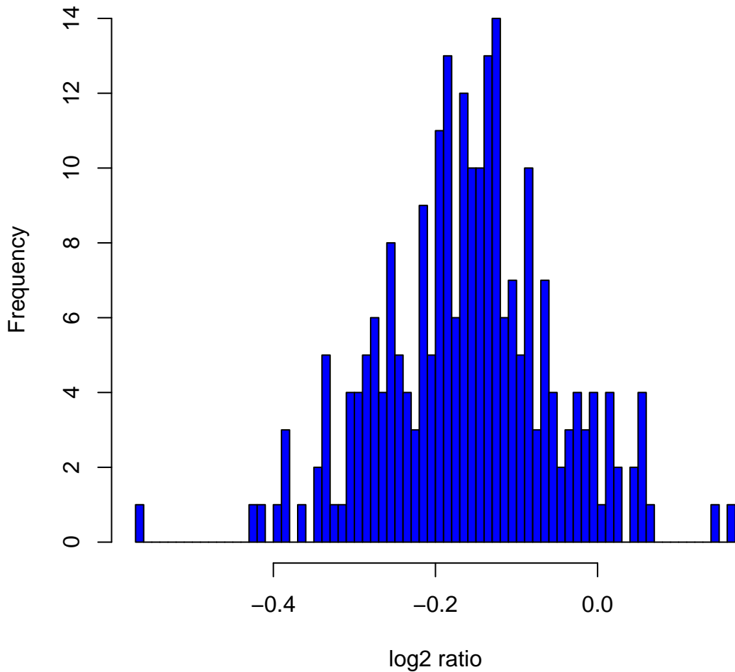
Histogram of log2ratios in 270 HapMap samples at clone Chr20tp-6E12
