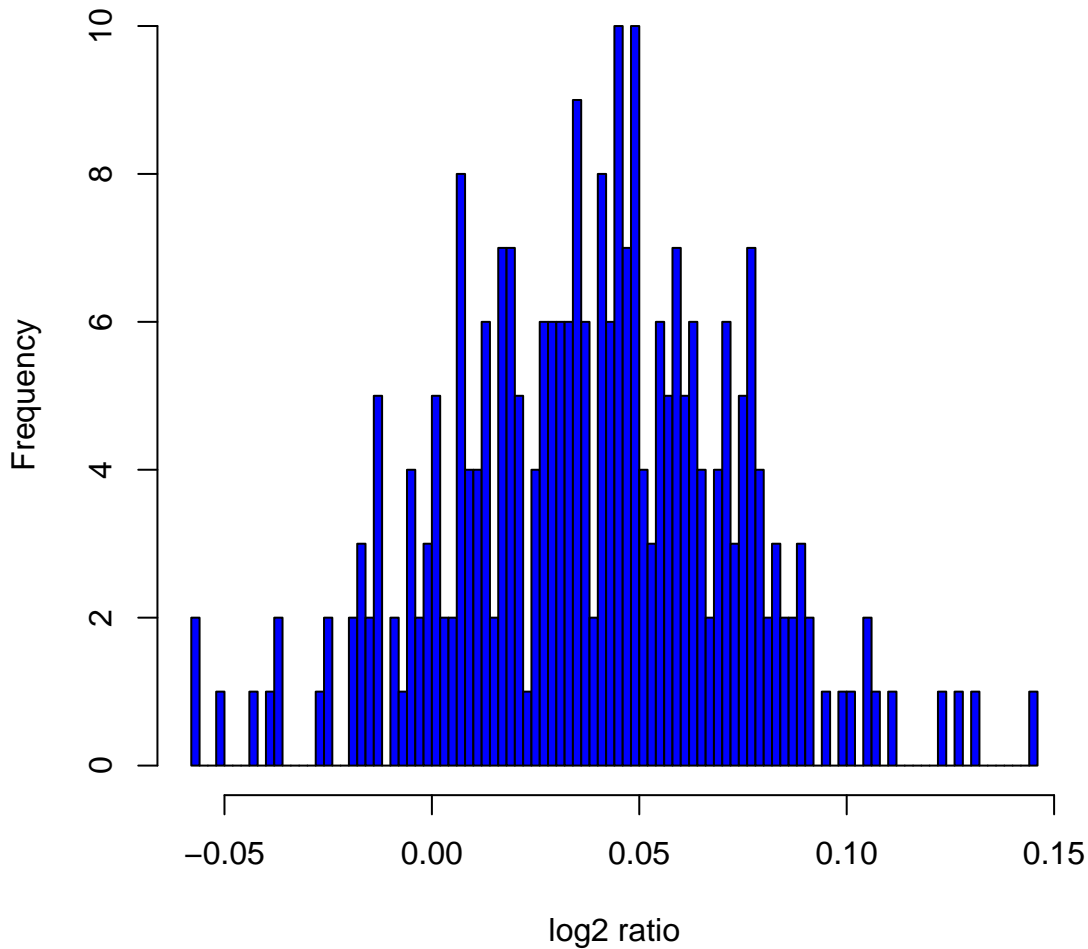
Histogram of log 2 ratios in 270 HapMap samples at clone Chr20tp-6G5
