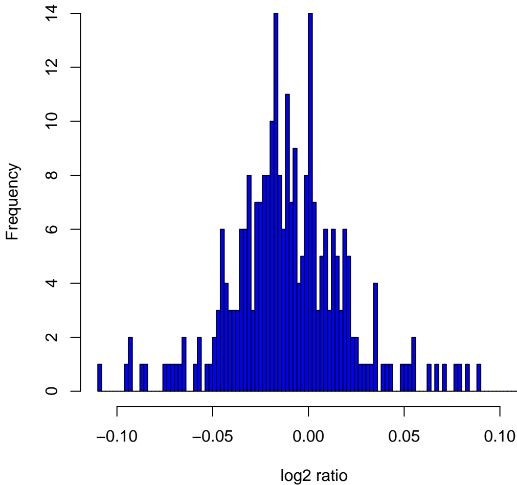
Histogram of log 2 ratios in 270 HapMap samples at clone Chr20tp-6G8
