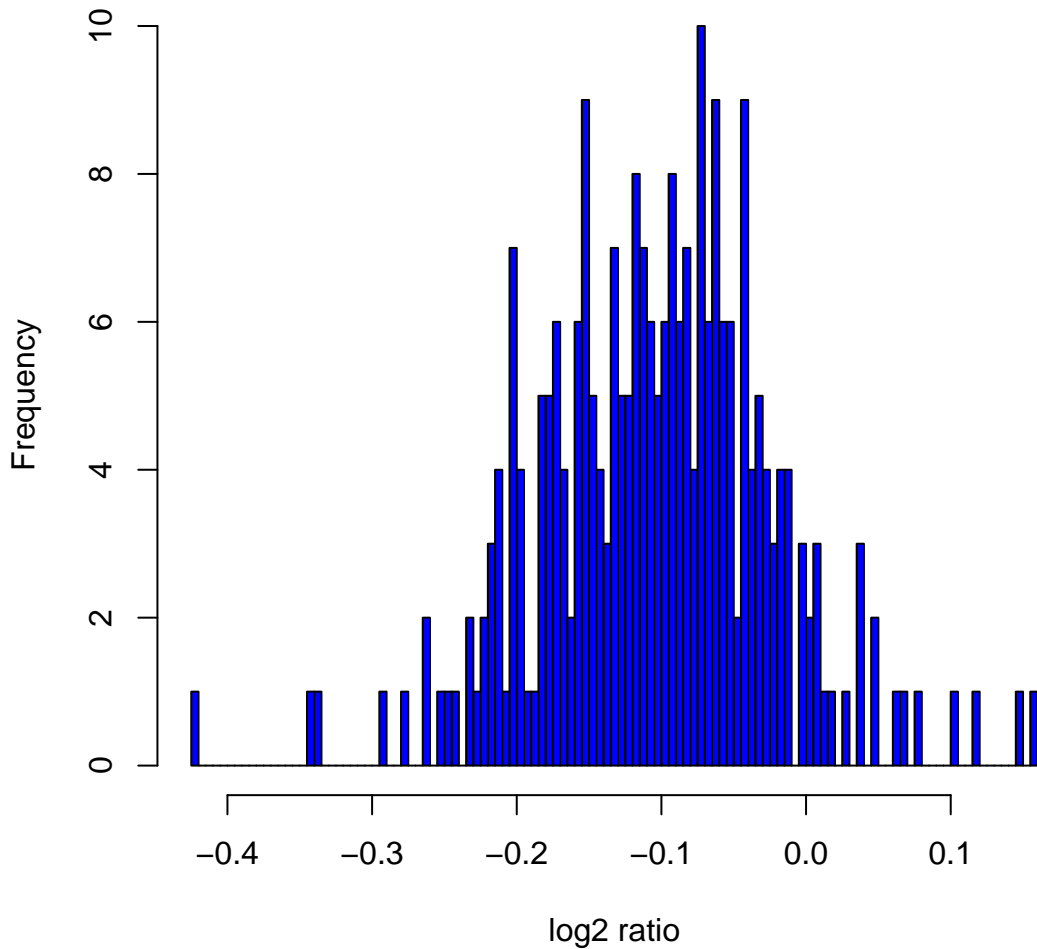
Histogram of log 2 ratios in 270 HapMap samples at clone Chr20tp-7A1
