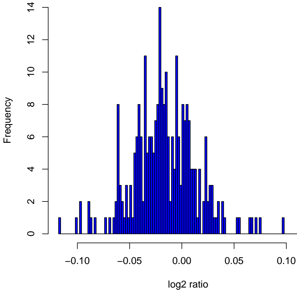
Histogram of log 2 ratios in 270 HapMap samples at clone Chr20tp-7B7
