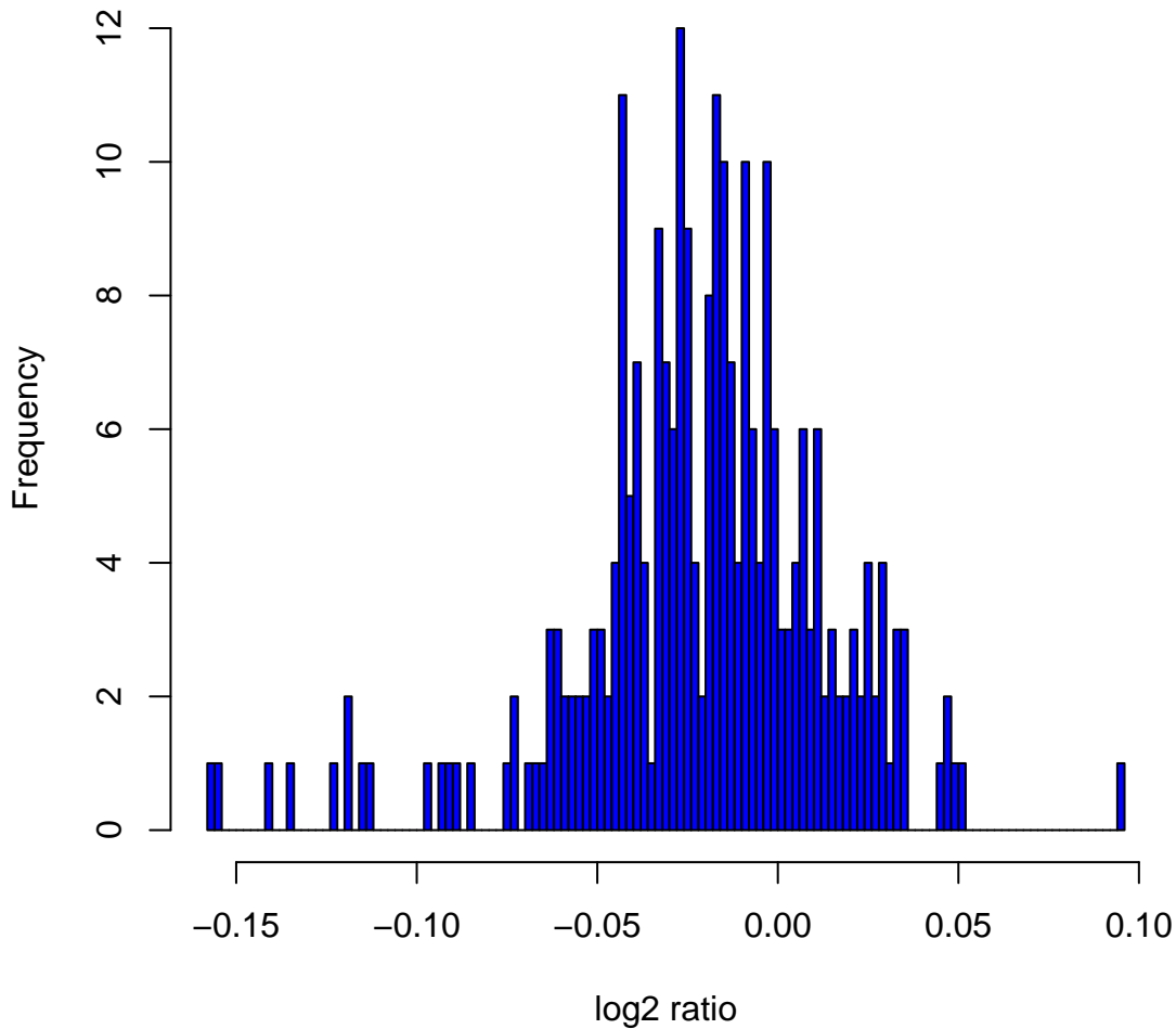
Histogram of log 2 ratios in 270 HapMap samples at clone Chr20tp-7C3
