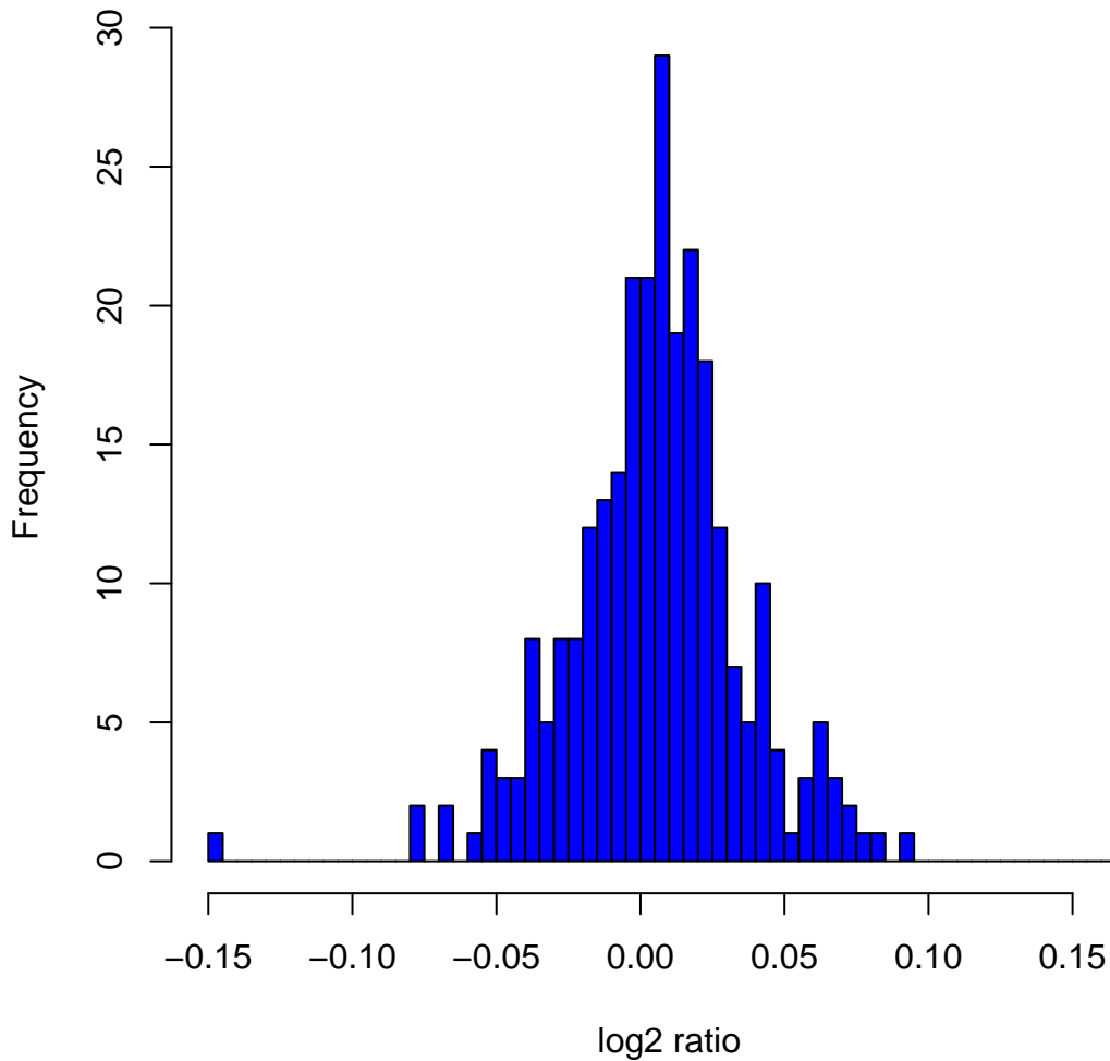
Histogram of log 2 ratios in 270 HapMap samples at clone Chr20tp-8A2
