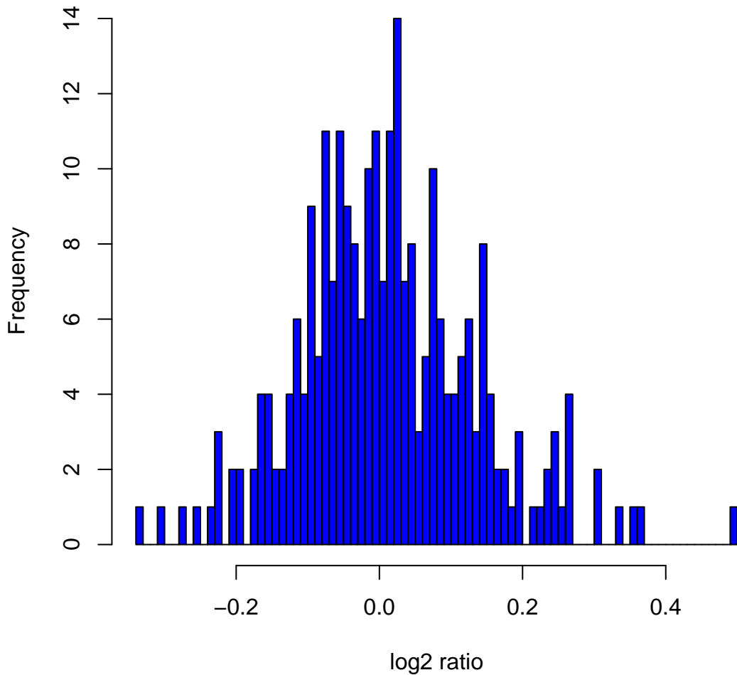
Histogram of log 2 ratios in 270 HapMap samples at clone Chr21tp-1B8
