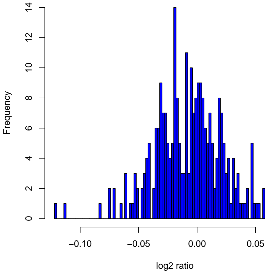
Histogram of log 2 ratios in 270 HapMap samples at clone Chr21tp-1C3
