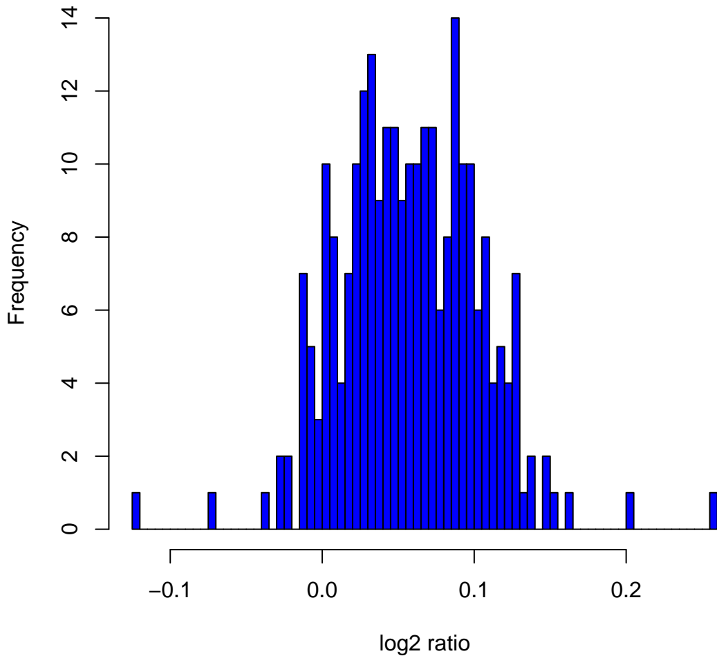
Histogram of log 2 ratios in 270 HapMap samples at clone Chr21tp-1D6
