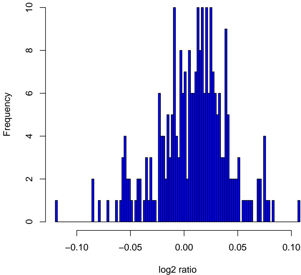
Histogram of log2ratios in 270 HapMap samples at clone Chr21tp-1F3
