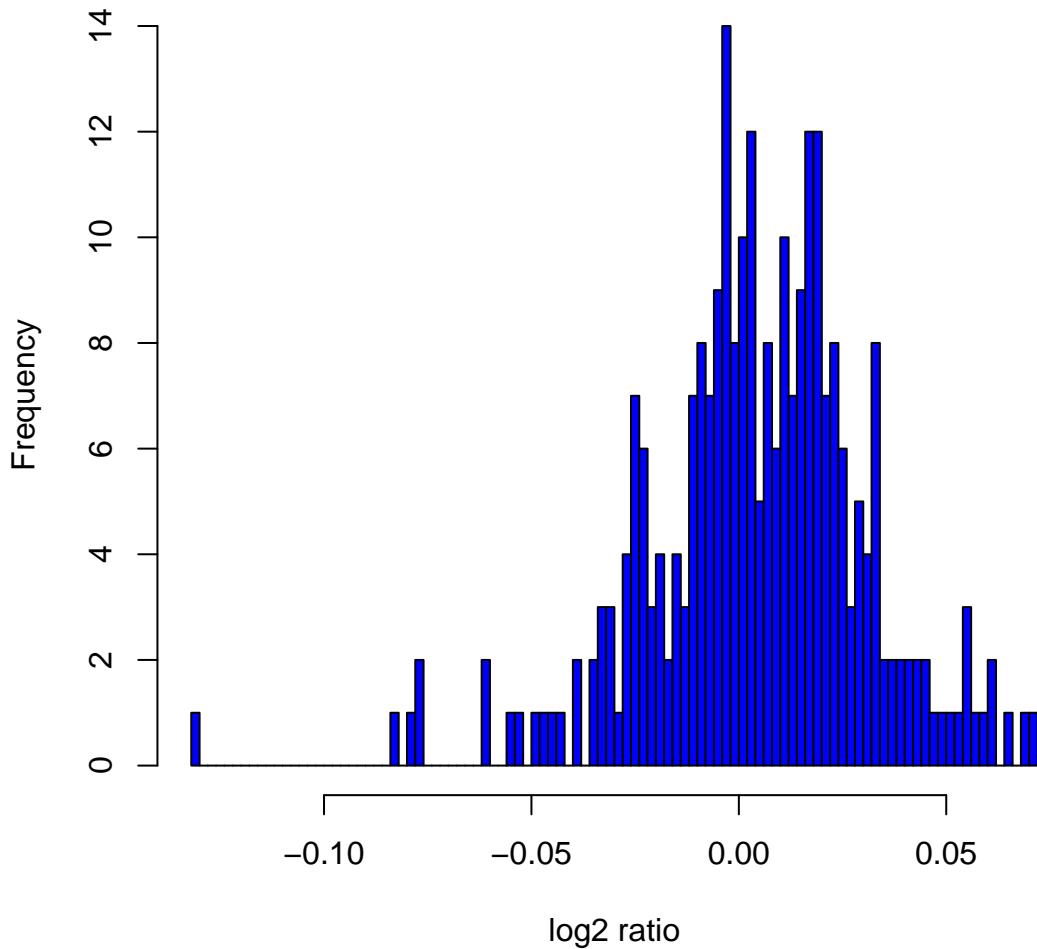
Histogram of log2ratios in 270 HapMap samples at clone Chr21tp-1G10
