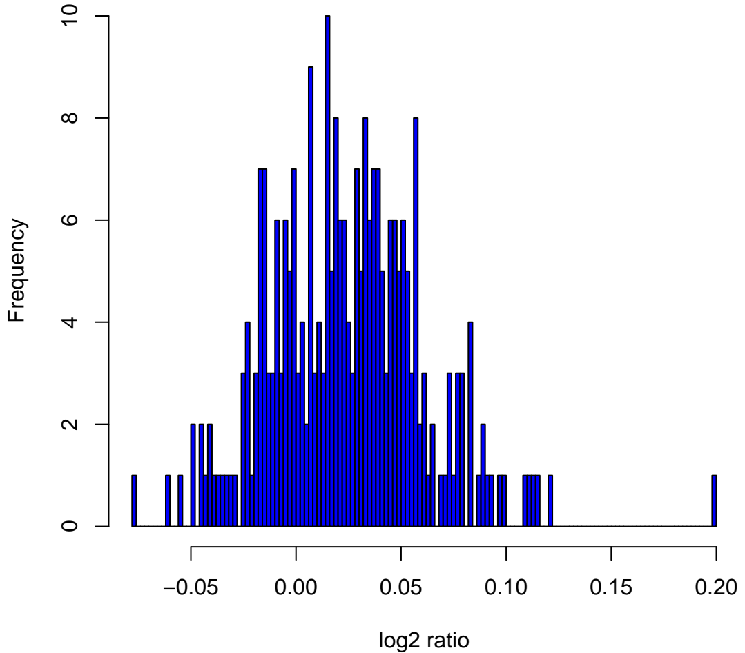
Histogram of log 2 ratios in 270 HapMap samples at clone Chr21tp-2C5
