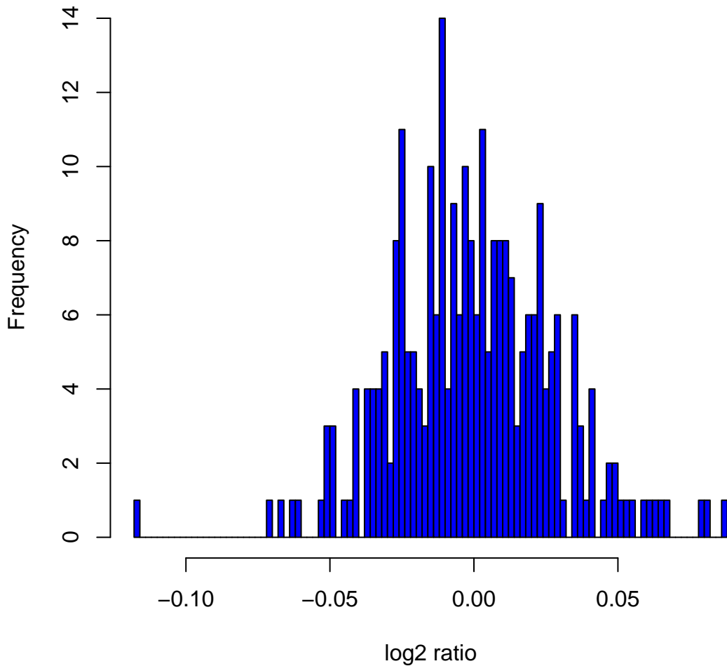
Histogram of log 2 ratios in 270 HapMap samples at clone Chr21tp-2H4
