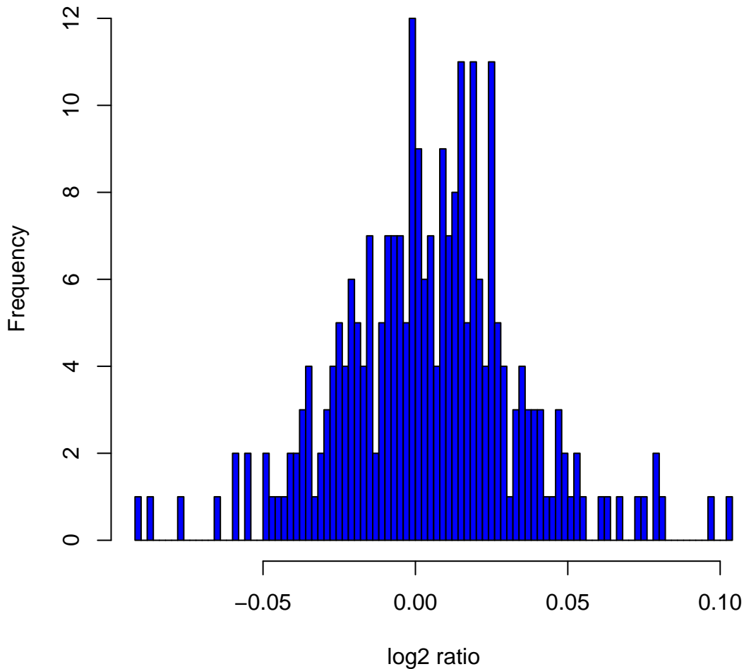
Histogram of log 2 ratios in 270 HapMap samples at clone Chr21tp-3B3
