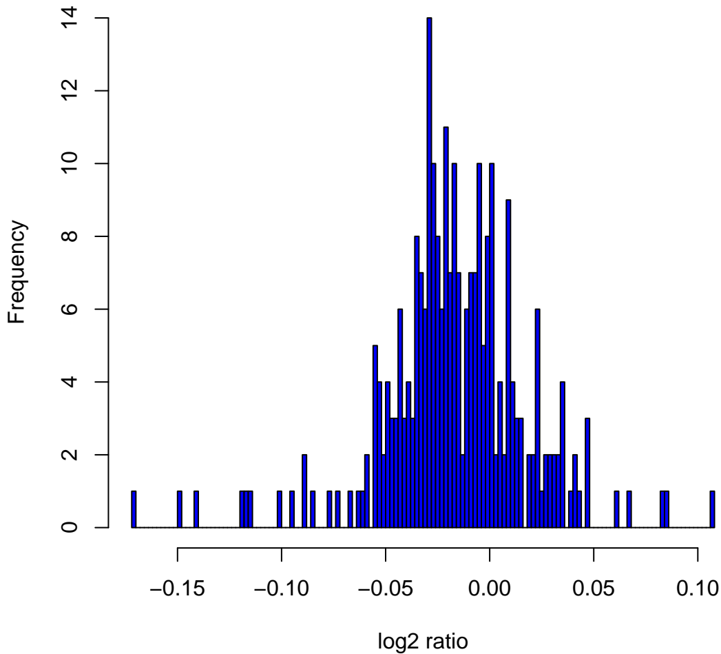
Histogram of log 2 ratios in 270 HapMap samples at clone Chr21tp-3D3
