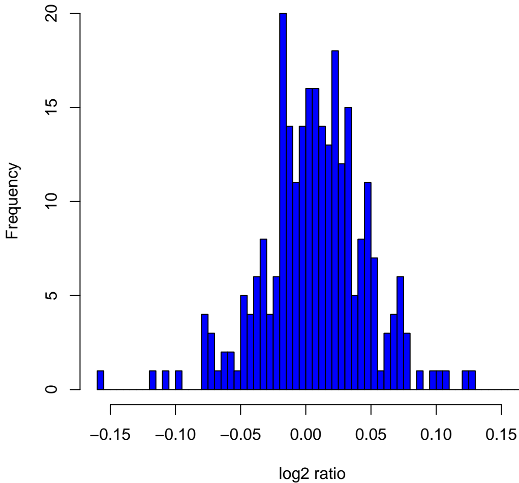
Histogram of log 2 ratios in 270 HapMap samples at clone Chr21tp-3E1
