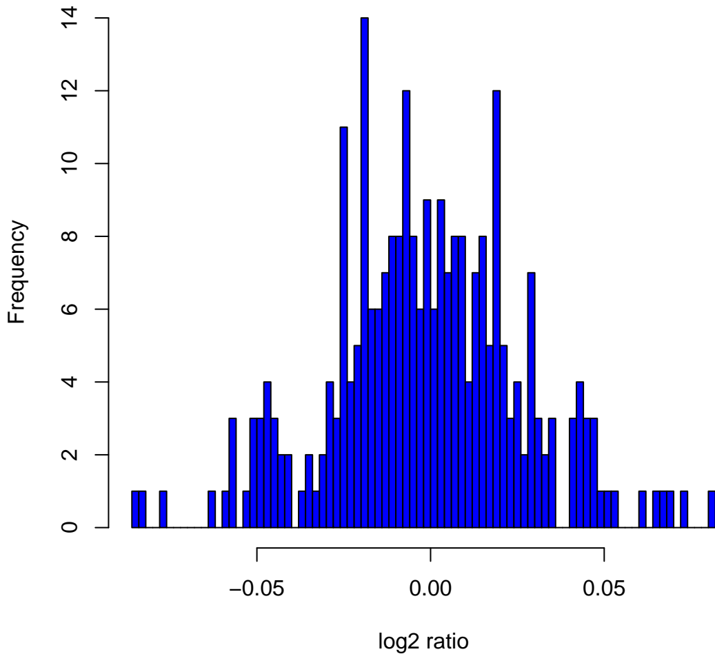
Histogram of \log_2 ratios in 270 HapMap samples at clone Chr21tp-3E4
