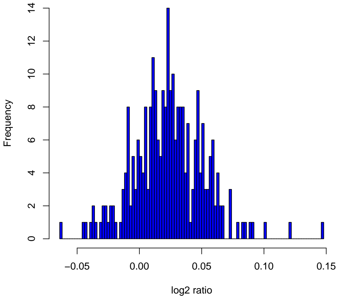
Histogram of log 2 ratios in 270 HapMap samples at clone Chr21tp-3F1
