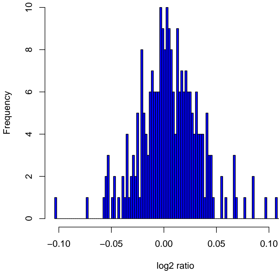
Histogram of log 2 ratios in 270 HapMap samples at clone Chr7tp-21E7
