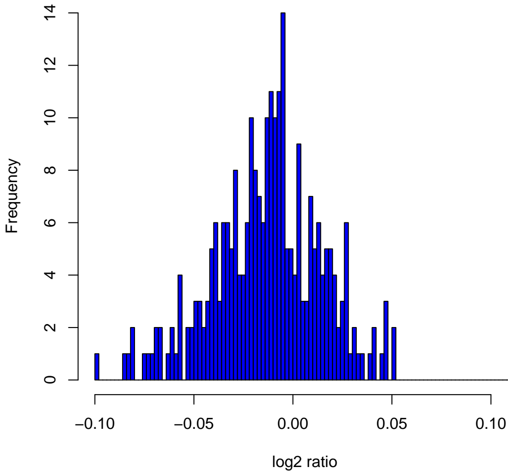
Histogram of log2ratios in 270 HapMap samples at clone Chr2tp-10D2
