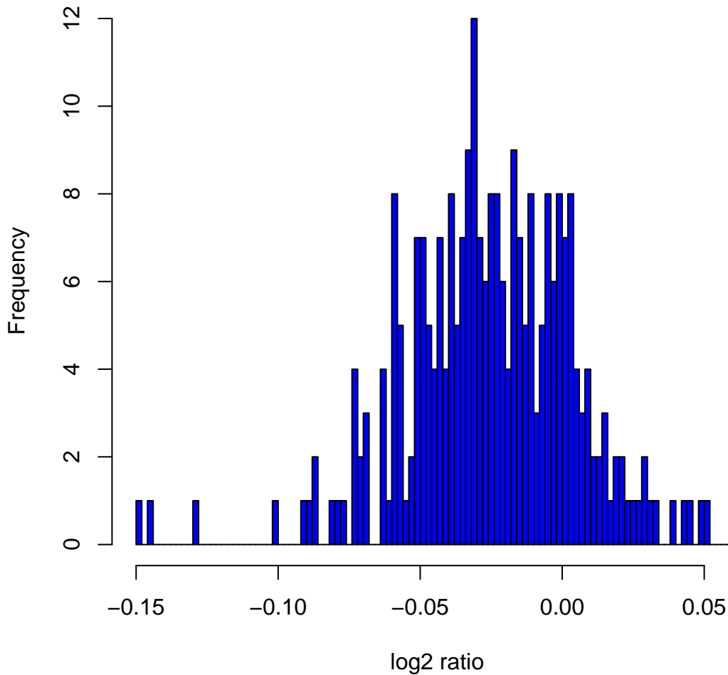
Histogram of log 2 ratios in 270 HapMap samples at clone Chr2tp-10F7
