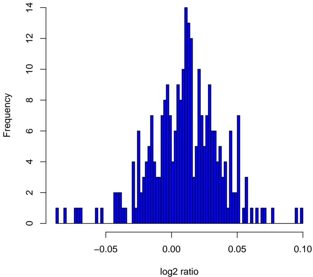
Histogram of log 2 ratios in 270 HapMap samples at clone Chr2tp-10G5
