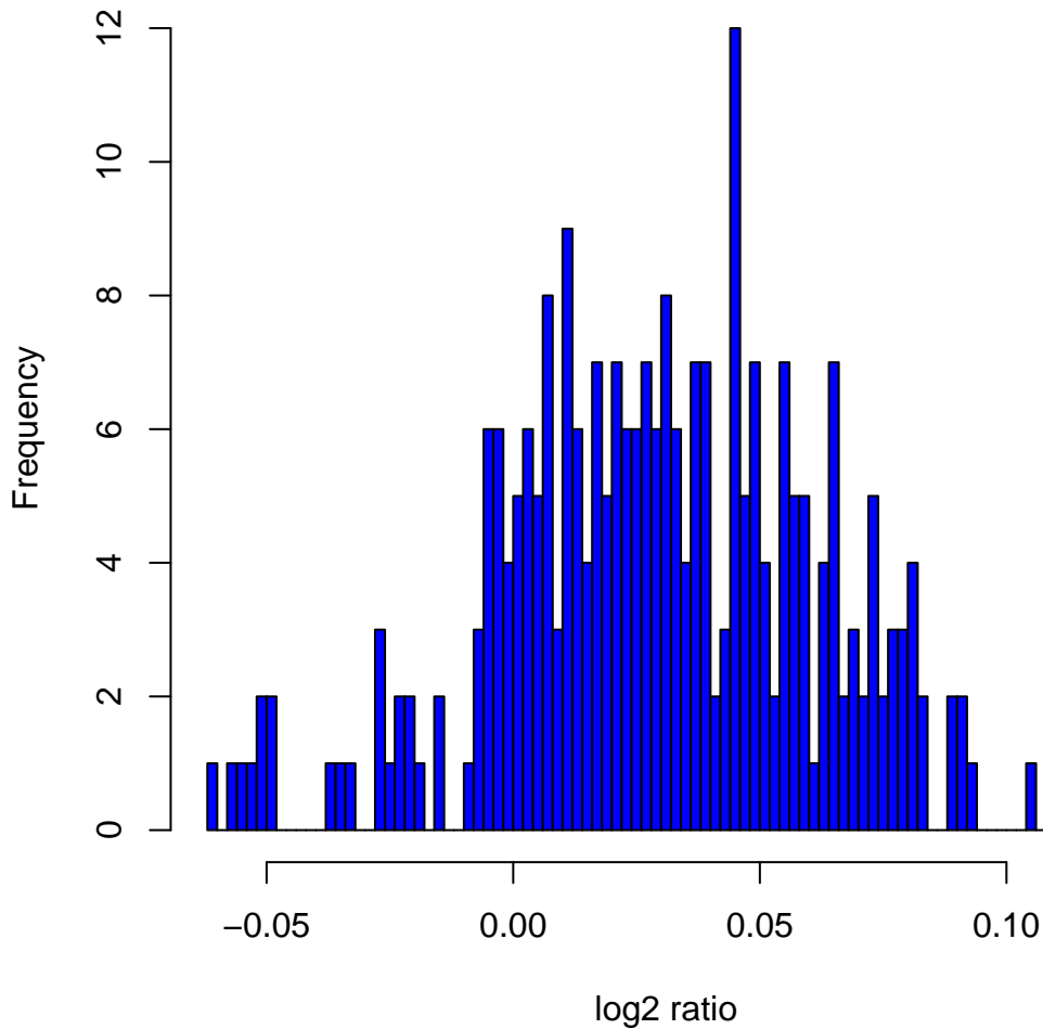
Histogram of log 2 ratios in 270 HapMap samples at clone Chr2tp-10G7
