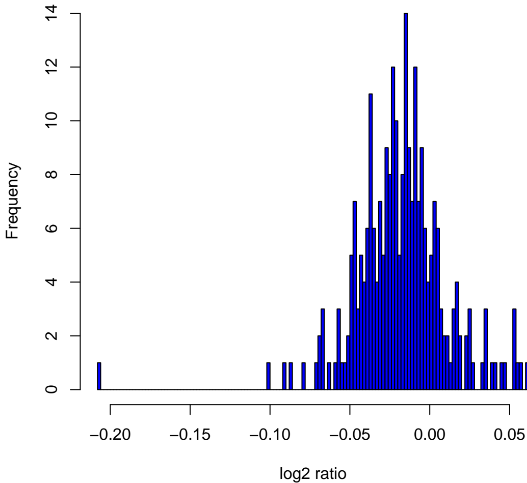
Histogram of log 2 ratios in 270 HapMap samples at clone Chr2tp-10G8
