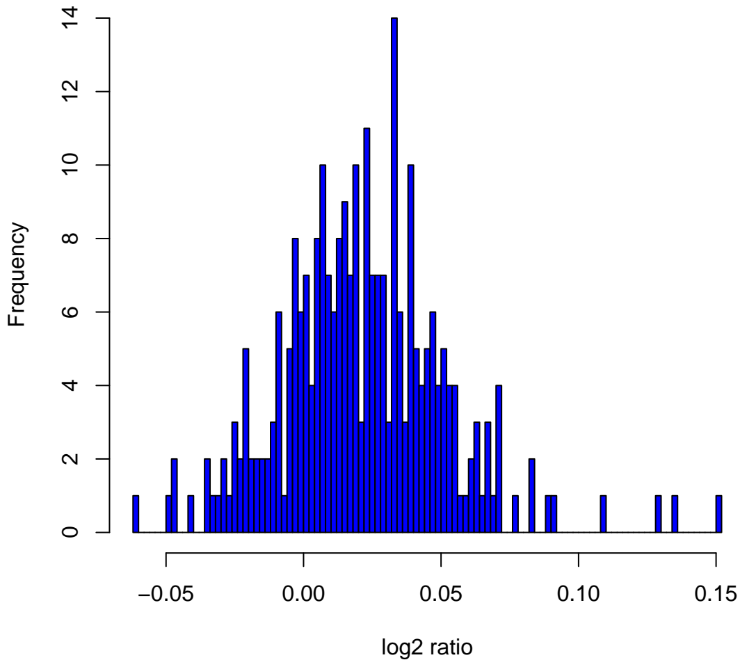
Histogram of log2ratios in 270 HapMap samples at clone Chr2tp-10H12
