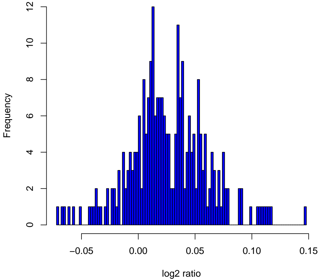
Histogram of log 2 ratios in 270 HapMap samples at clone Chr2tp-11D6
