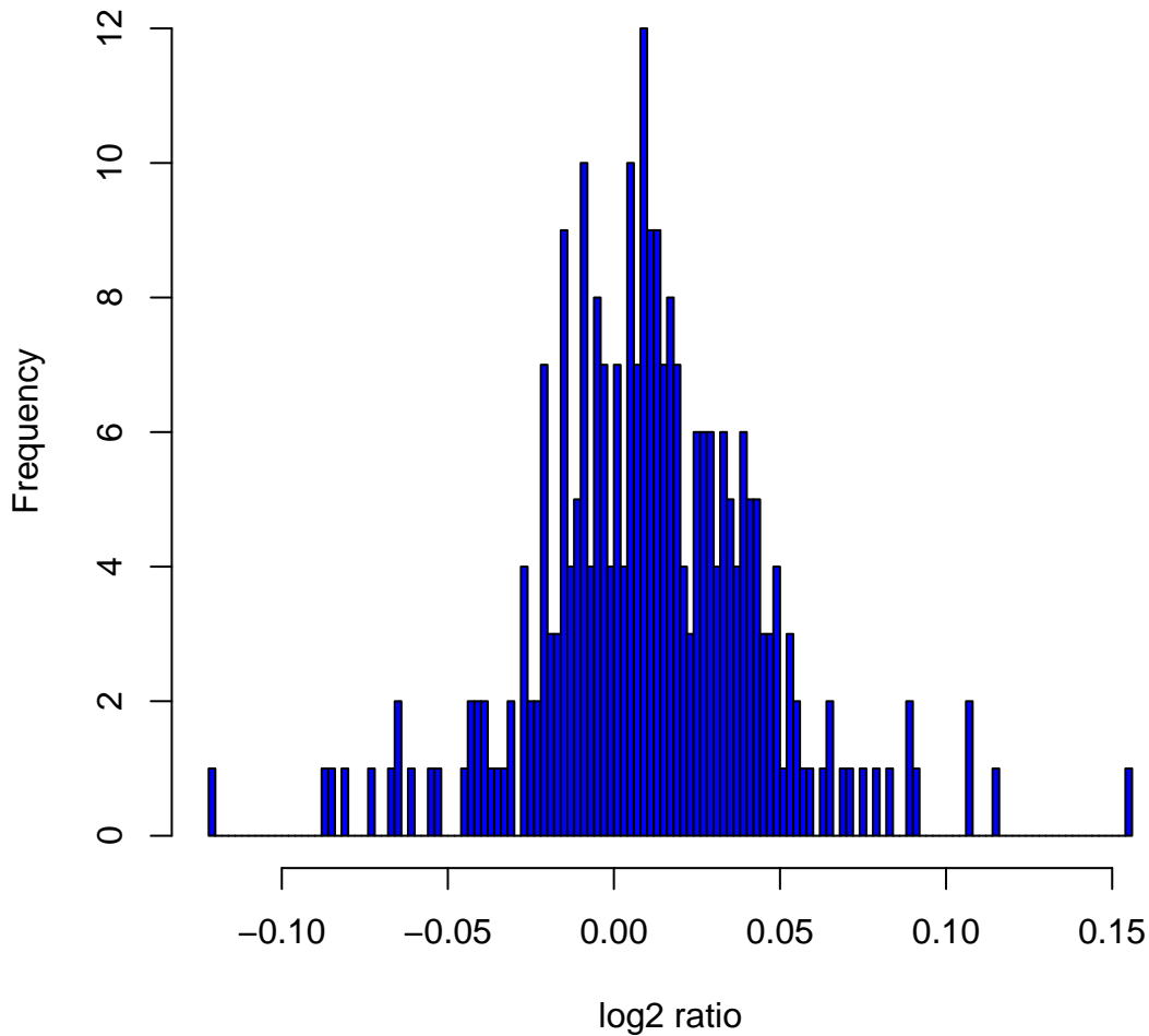
Histogram of \log_2 ratios in 270 HapMap samples at clone Chr2tp-11G9
