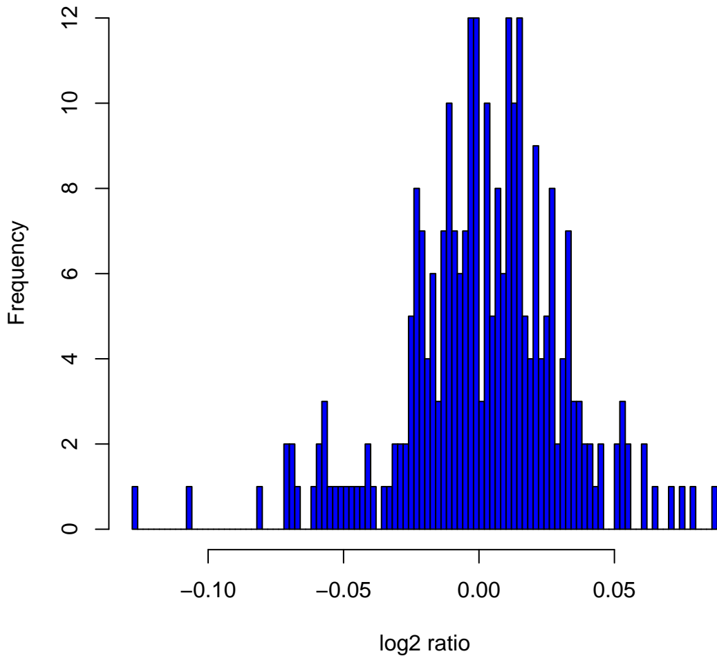
Histogram of log 2 ratios in 270 HapMap samples at clone Chr2tp-12C2
