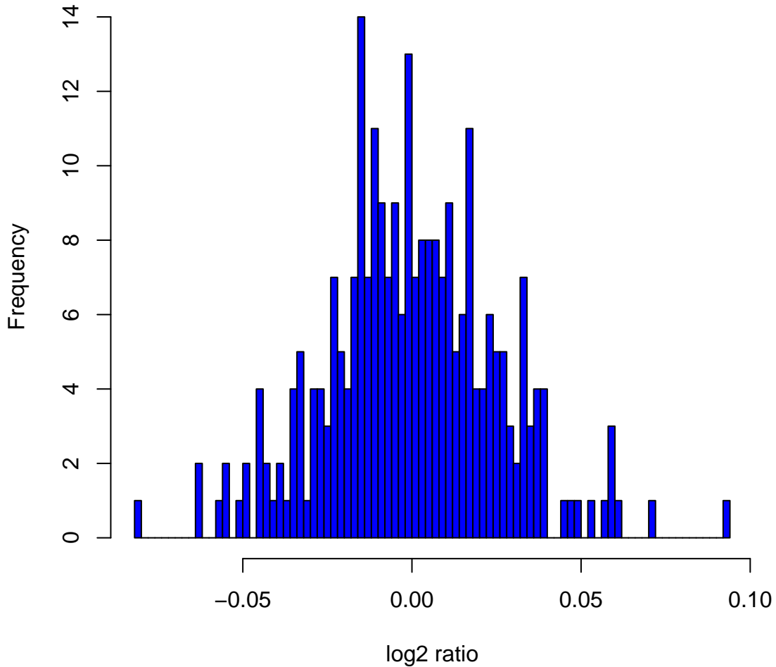
Histogram of log2ratios in 270 HapMap samples at clone Chr2tp-12E10
