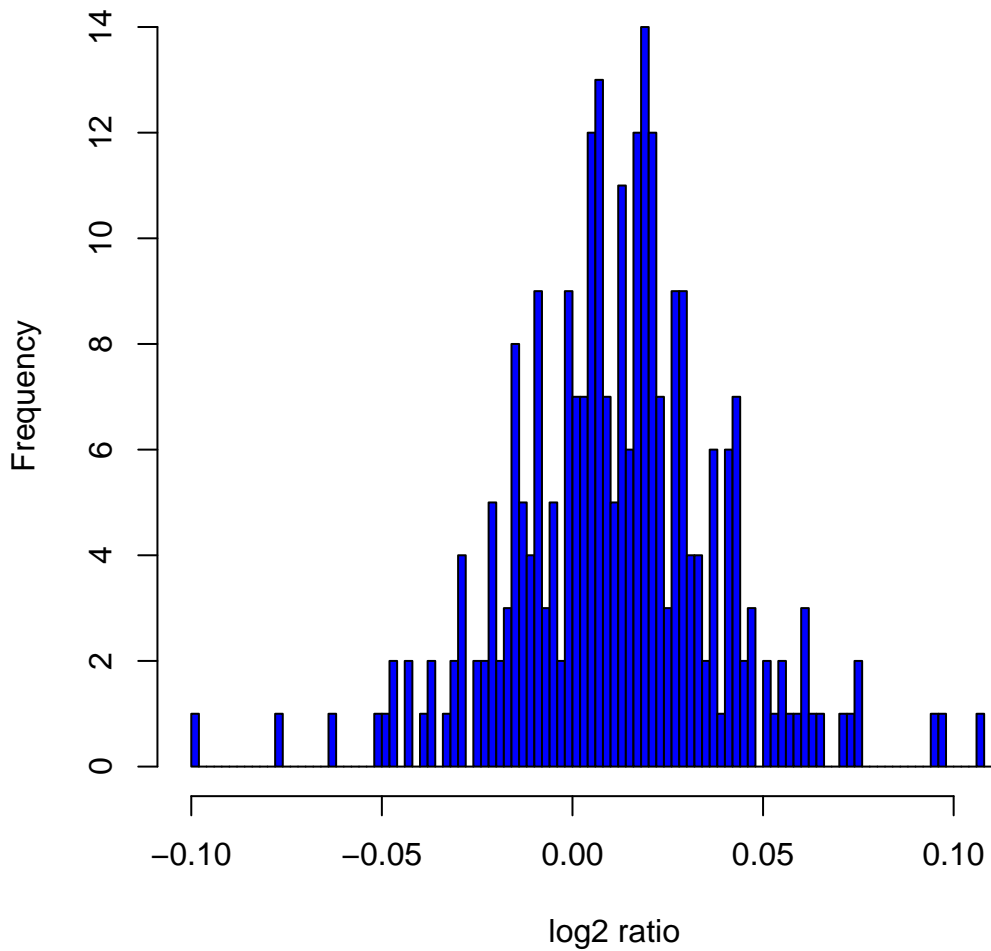
Histogram of log 2 ratios in 270 HapMap samples at clone Chr2tp-12E9
