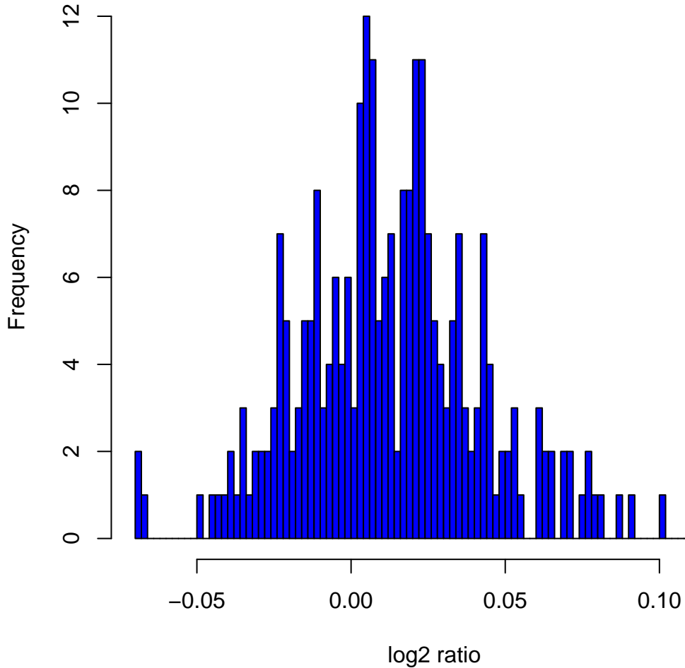
Histogram of log2ratios in 270 HapMap samples at clone Chr2tp-12H11
