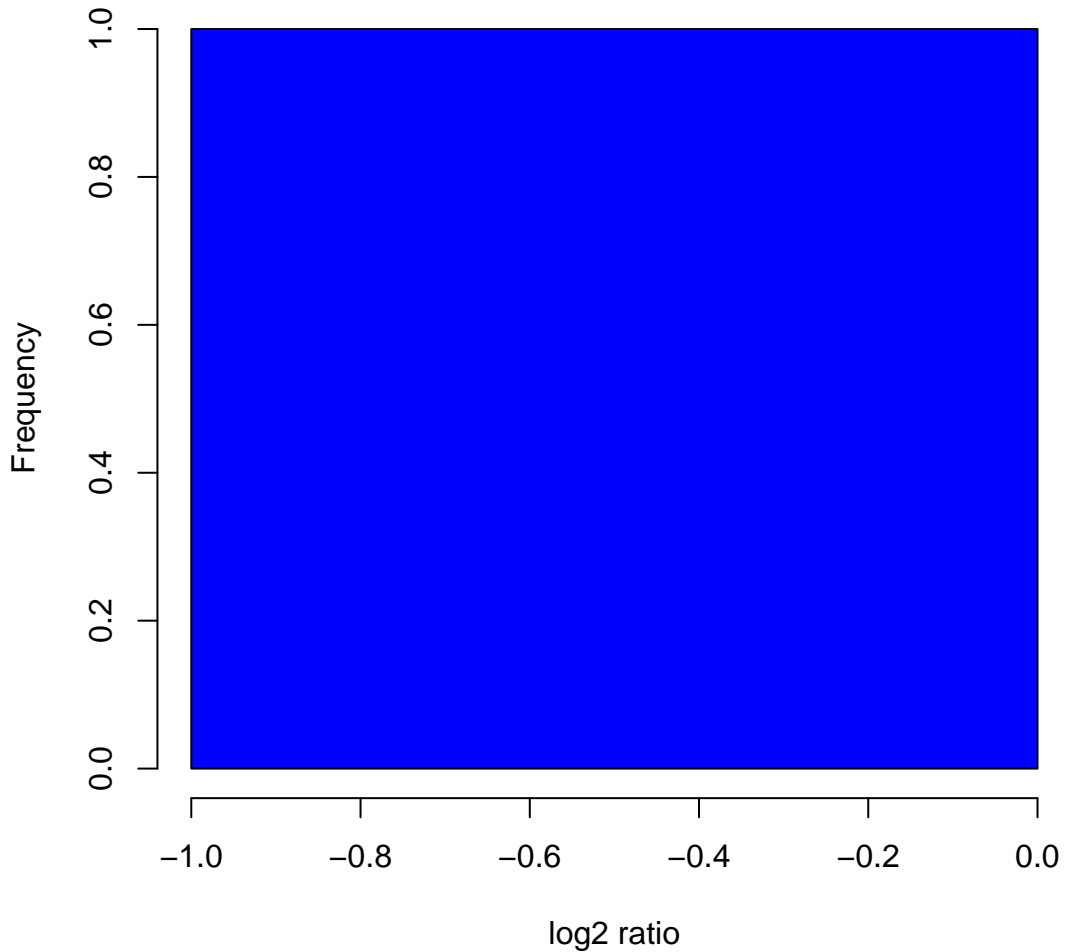
Histogram of log 2 ratios in 270 HapMap samples at clone Chr2tp-13A11
