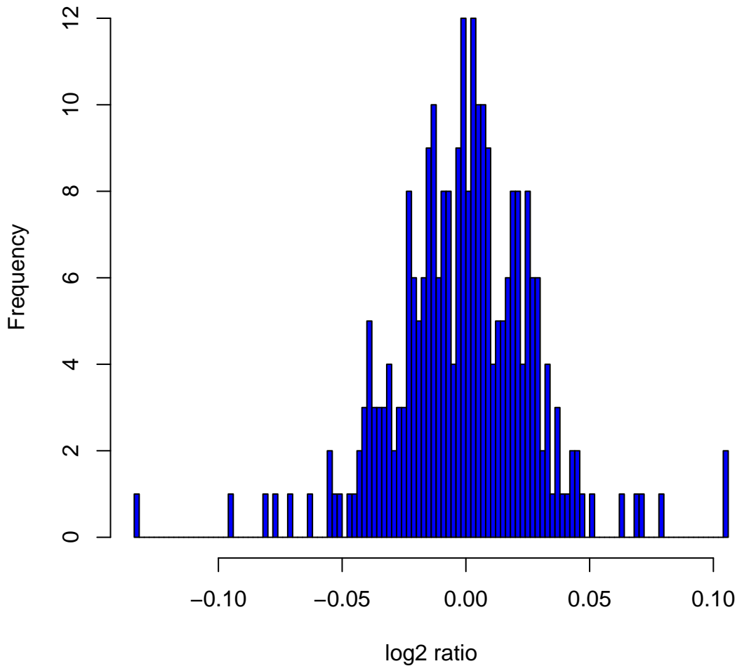
Histogram of log 2 ratios in 270 HapMap samples at clone Chr2tp-13A6
